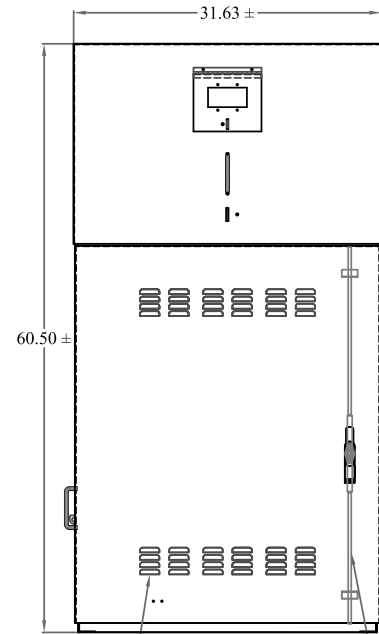
LOUVERED DOOR (STANDARD) FRONT VIEW
