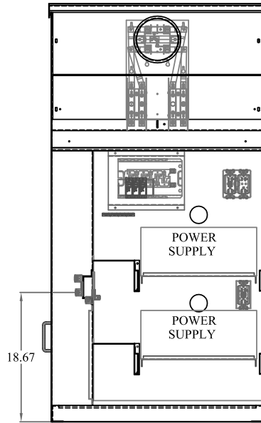
FRONT VIEW SHOWN LESS CUSTOMER DOOR
